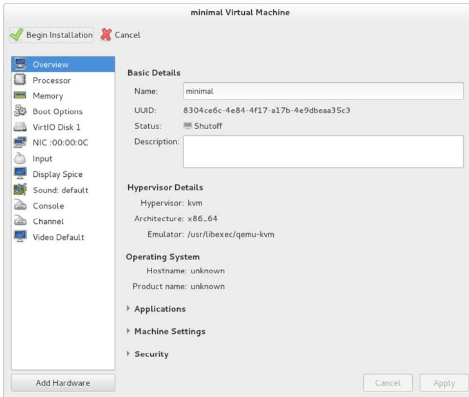
Figure 15.8: Create a virtual machine, customize configuration
