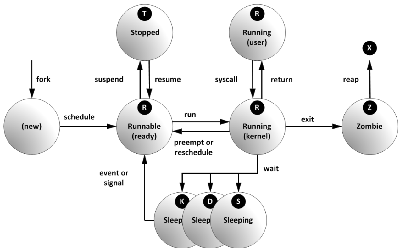
Figure 7.2: Linux process states
