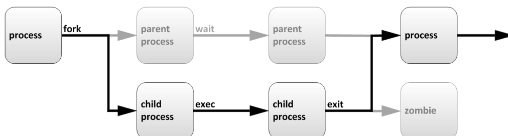
Figure 7.1: Process life cycle
