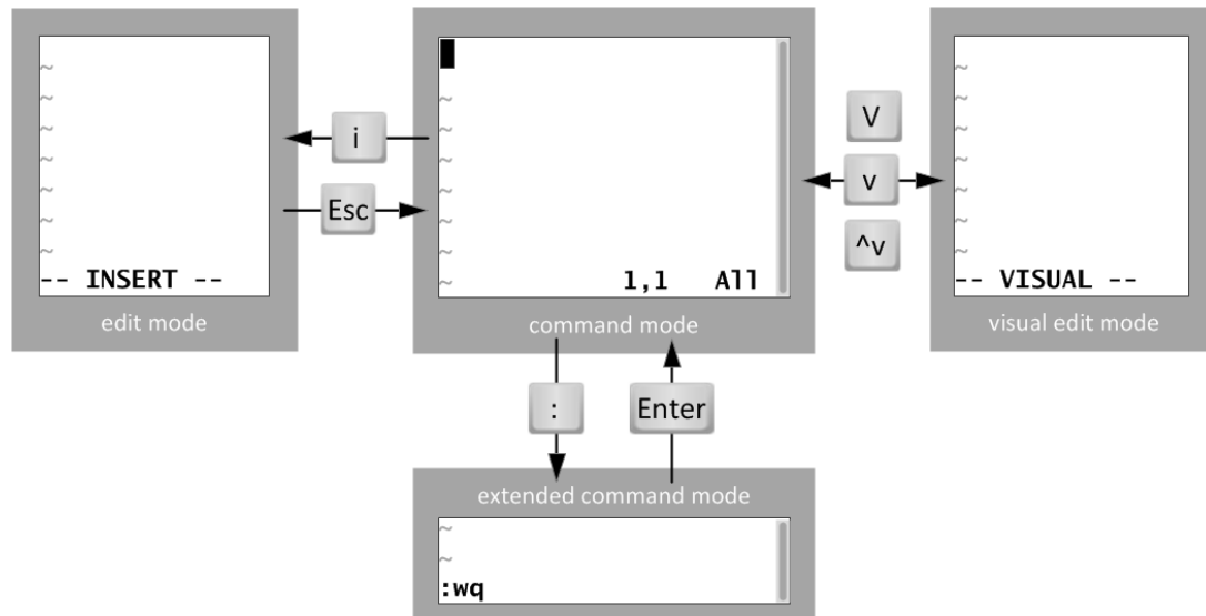
Figure 4.10: Moving between Vim modes
