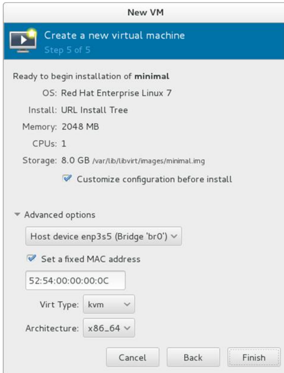
Figure 15.7: Create a virtual machine (step 5 of 5)
