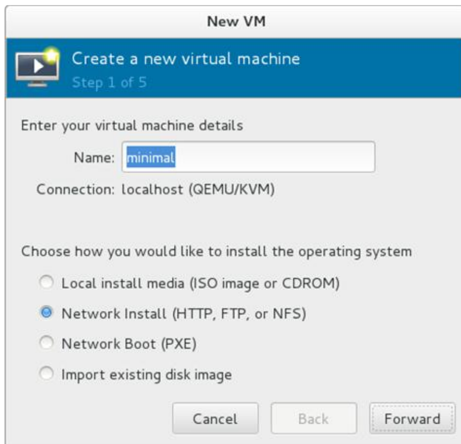
Figure 15.3: Create a virtual machine (step 1 of 5)
