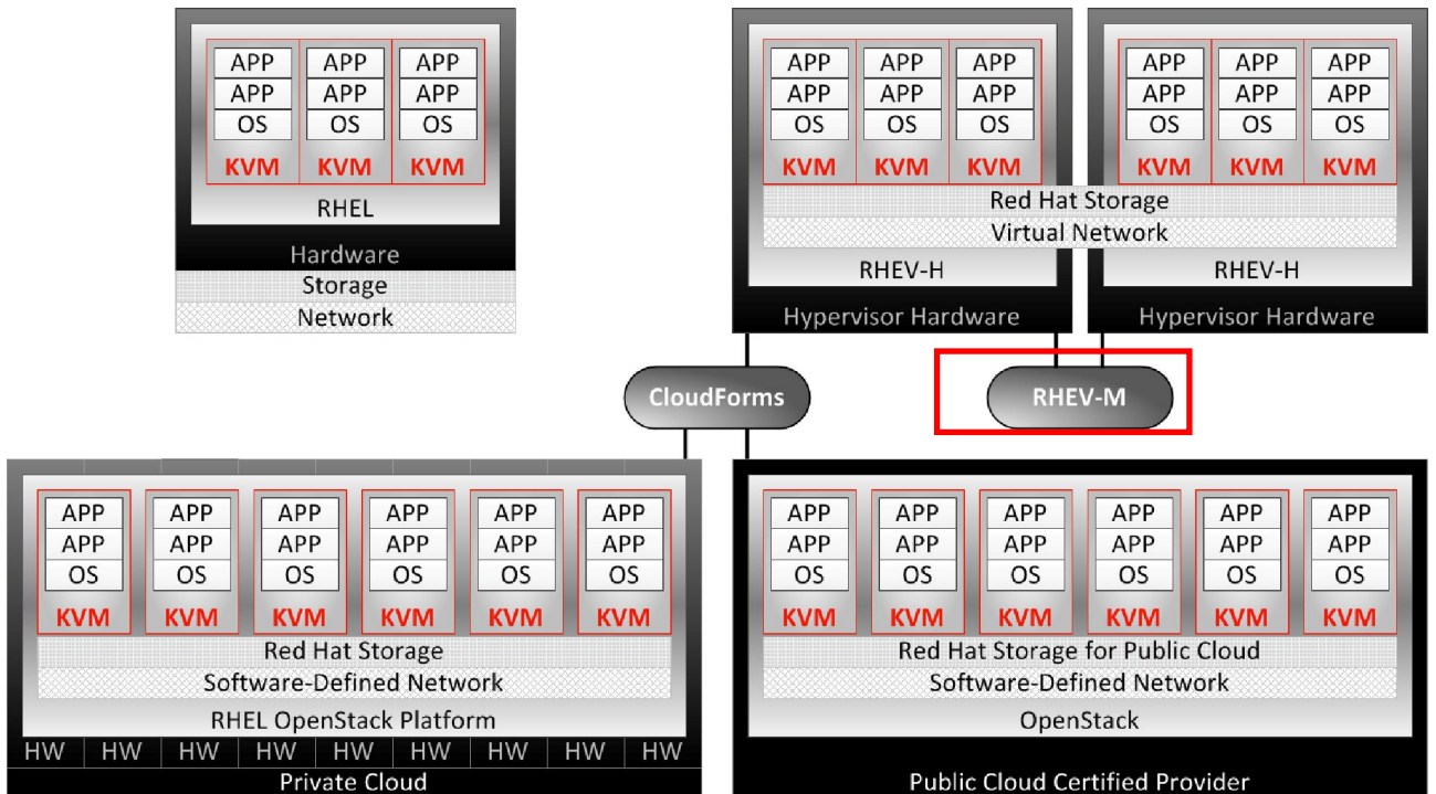
Figure 15.1: KVM throughout the Red Hat cloud infrastructure
