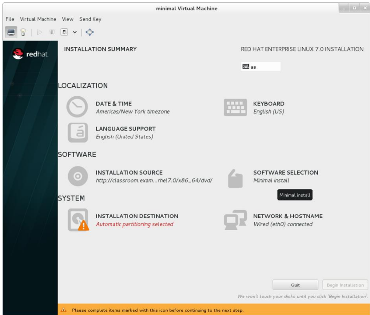
Figure 15.9: Anaconda installer, installation summary
